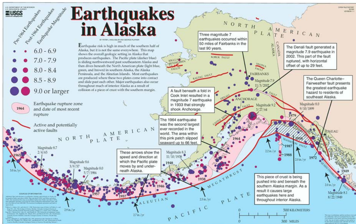
Alaskan seismicity: faults, earthquakes, and rupture zones
