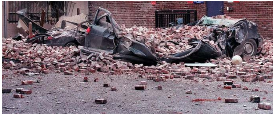
Nisqually earthquake damage at a building without seismic retrofit
