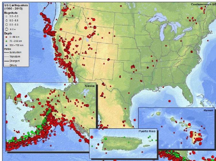
Sites of major earthquakes in the US
